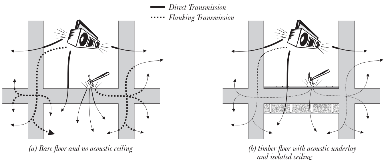
Figure 1 – Sound Transmission paths
